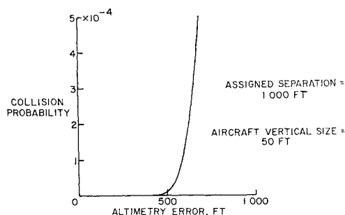
Fig. 4 Collision probability vs altimetry error.
