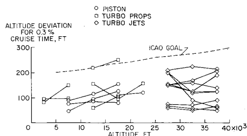
Fig. 2 Flight technical errors of 19 civil transports.
