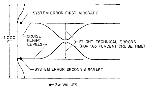
Fig. 5 Altimetry errors of two aircraft at 40,000 ft.
