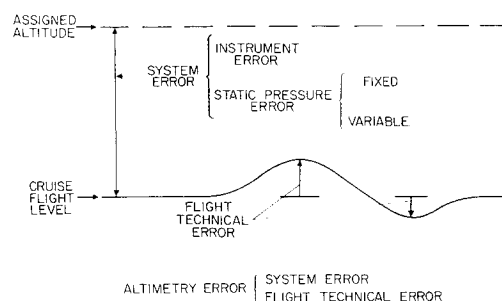
Fig. 1. Pressure altimetry errors.
